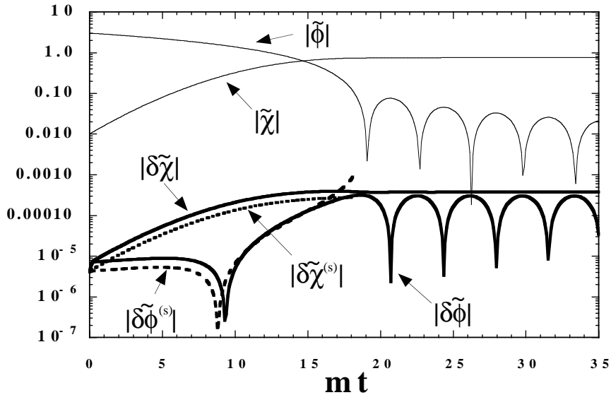
FIG. 2: The evolution of background fields, \tilde{\phi} = \phi/m_{\text{pl}} and \tilde{\chi} = \chi/m_{\text{pl}} , and large-scale field perturbations, \delta\tilde{\phi} \equiv k^{3/2}\delta\phi/m_{\text{pl}} and \delta\tilde{\chi} \equiv k^{3/2}\delta\chi/m_{\text{pl}} , in the massive chaotic inflationary scenario with a non-minimally coupled \chi field for \xi = -0.02 . The initial values of scalar fields are chosen as \phi_* = 3m_{\text{pl}} and \chi_* = 10^{-2}m_{\text{pl}} . The slow-roll results of Eq. (4.33) are also plotted, where we denote \delta\tilde{\phi}^{(s)} and \delta\tilde{\chi}^{(s)} in the figure. We find that slow-roll approximations are valid except in the final stage of inflation ( mt > 17 ). The evolution of \delta\tilde{\phi}^{(s)} and \delta\tilde{\chi}^{(s)} after inflation is not shown.
